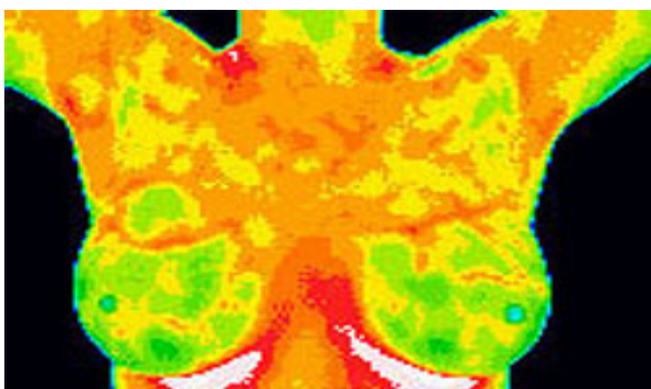
Before Treatment
